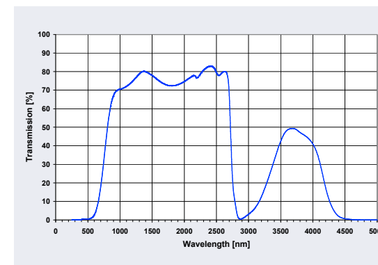
Radiation permeability of dark glass
